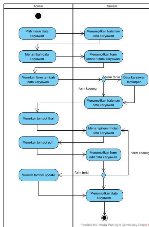
Gambar 3.2 Activity Diagram Karyawan
