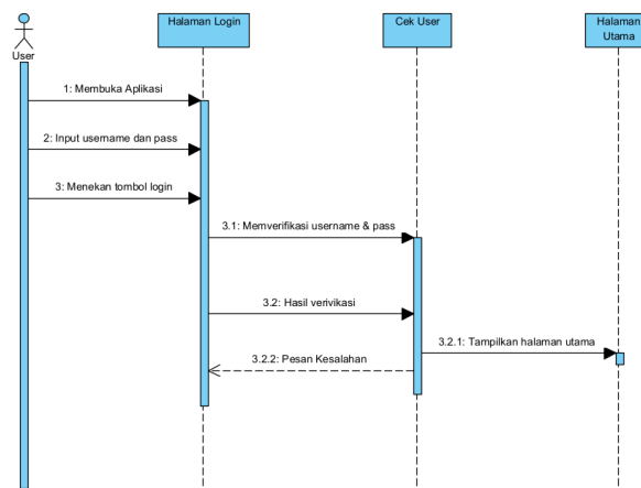
Gambar 3.4 Sequence Diagram Login
